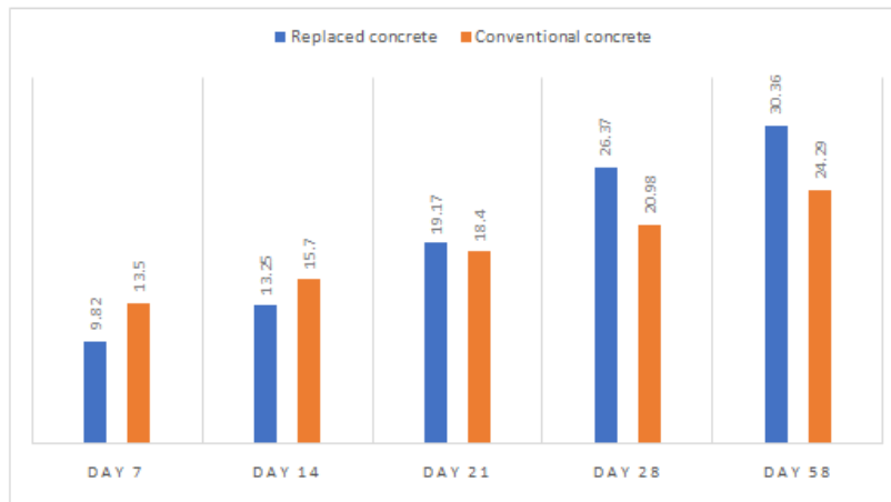
Fig. 2 Comparison of compressive strength of the conventional and replaced concrete
