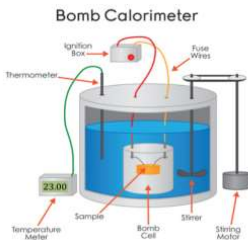
Figure 3. Bomb calorimeter
