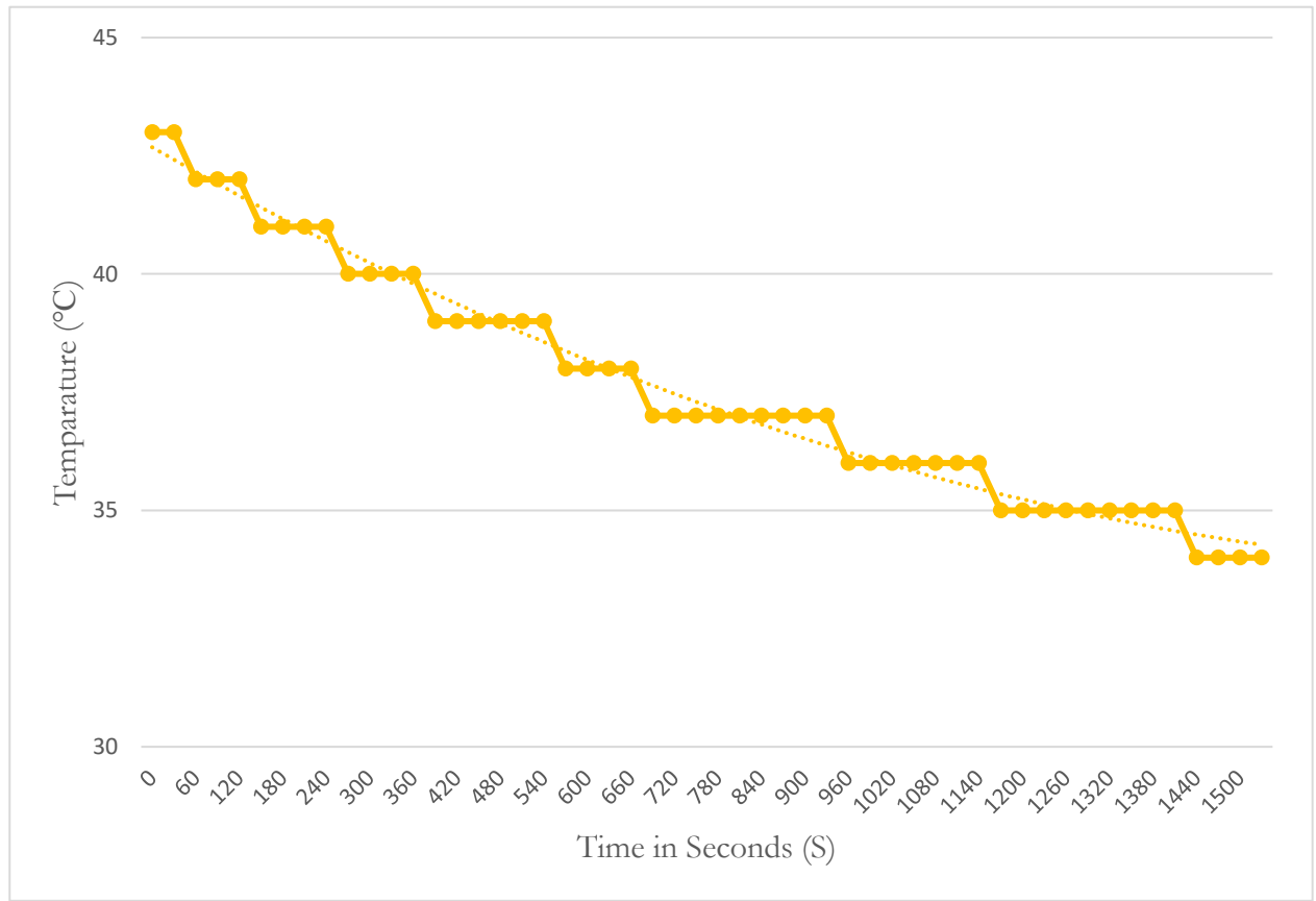
Figure 4; Cooling Curve for Grass
