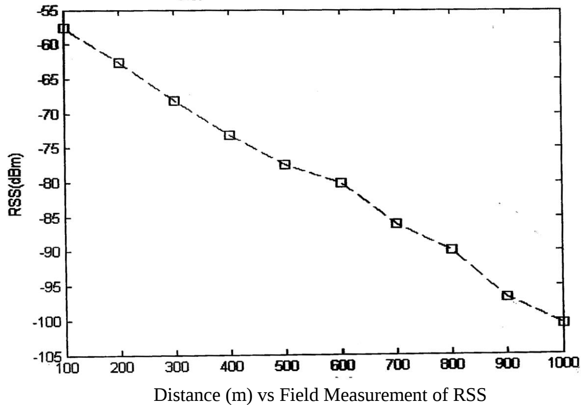
Figure 4.1 Received Signal Strength (RSS) vs Distance for the characterized environment (i.e experimental testbed)
