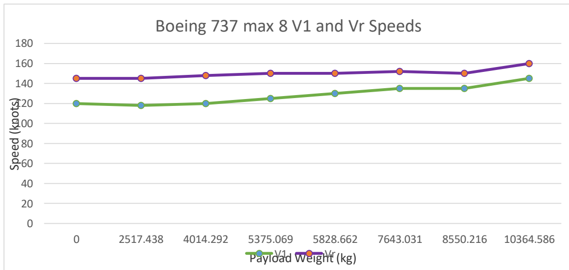
Graph 3.1.5 - V1 and V2 speeds comparison of Boeing 737 Max 8
