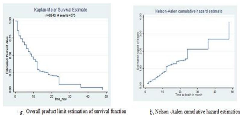
Fig. 1: Chart for Kaplan-Meier and Nelson Aalen Estimation
