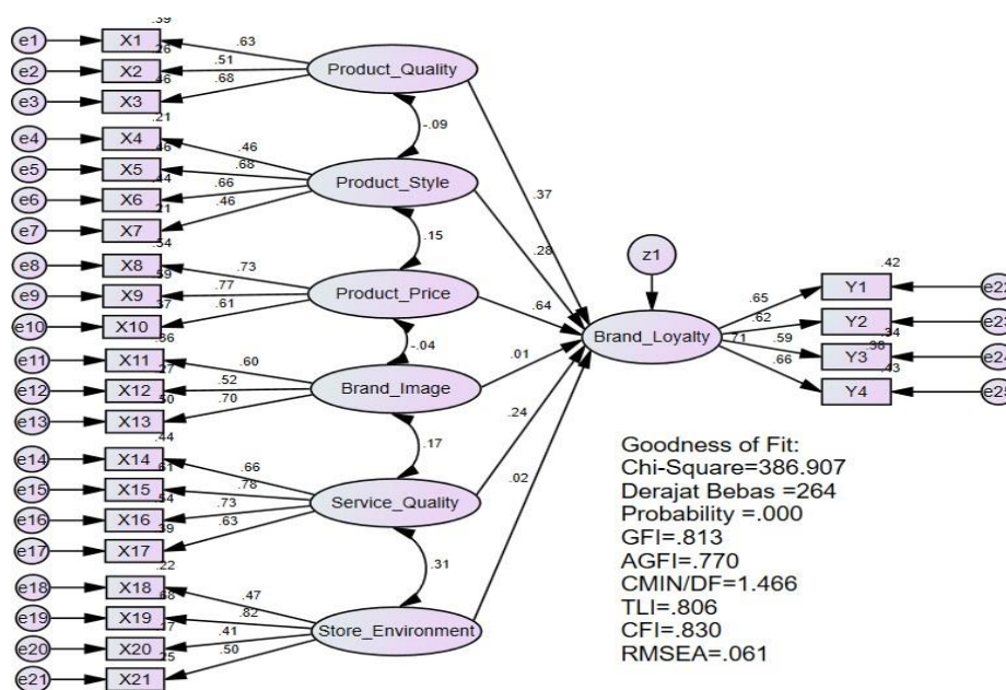
Figure 4.1: The Framework of Analysis Result
