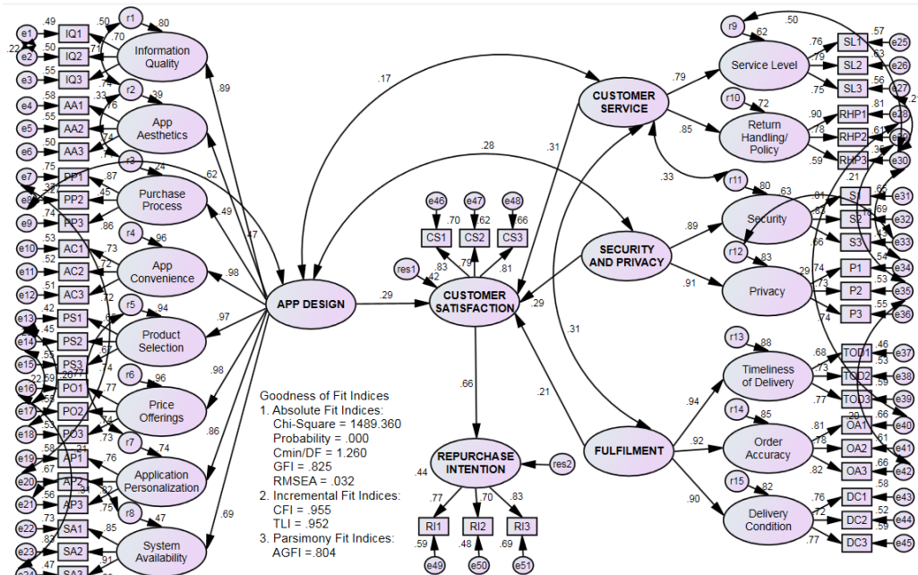
Figure 4.1 Full Structural Equation Model
