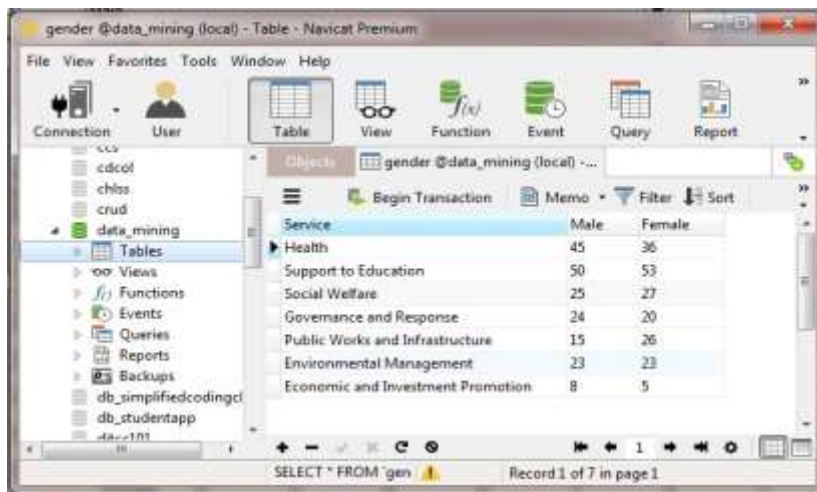
Figure 3. Datasets on Gender
