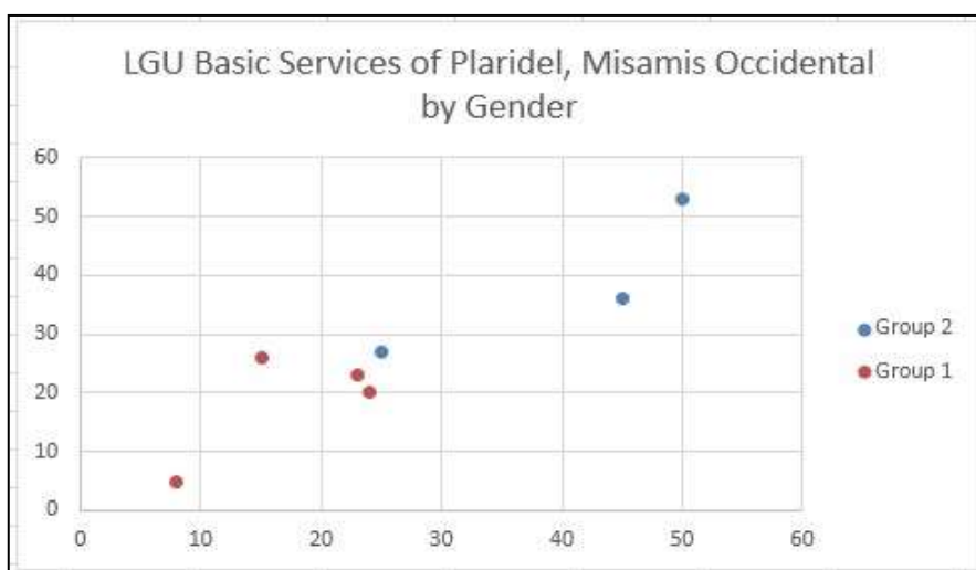
Figure 8. Scattered Plot by Gender
