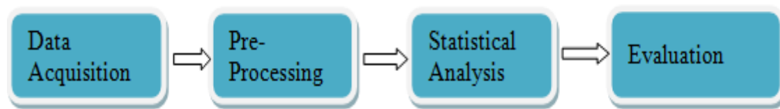
Figure 1: Overall methodology
