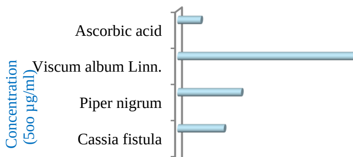
Fig. 2. IC 50 value of some plant extracts in comparison of standard ascorbic acid
