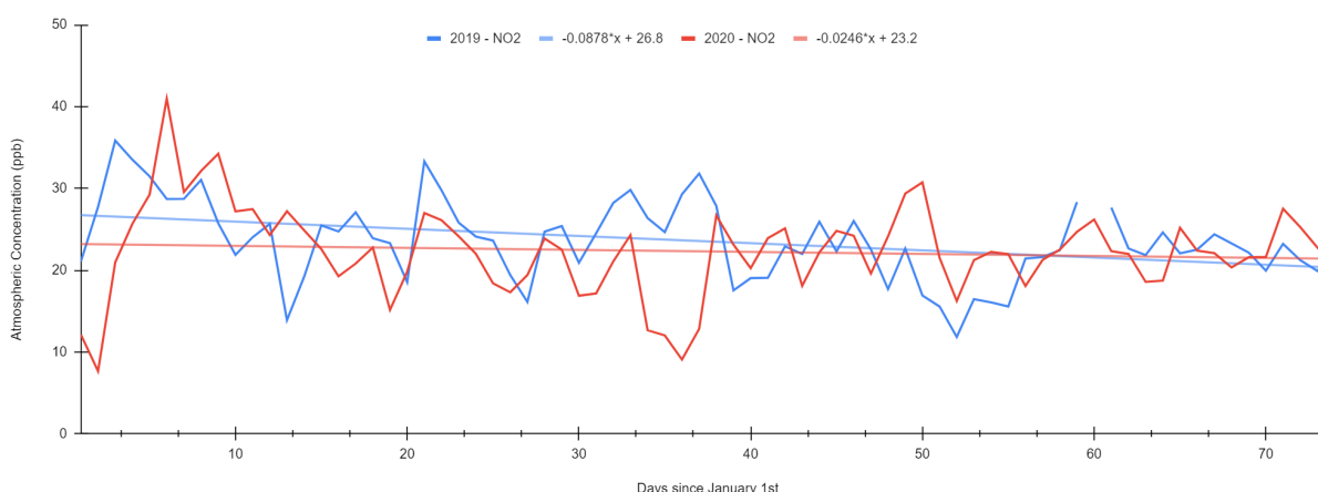
Daily averages of Nitrogen Dioxide in Mexico City from January 1st to March 14, 2020 and 2019
