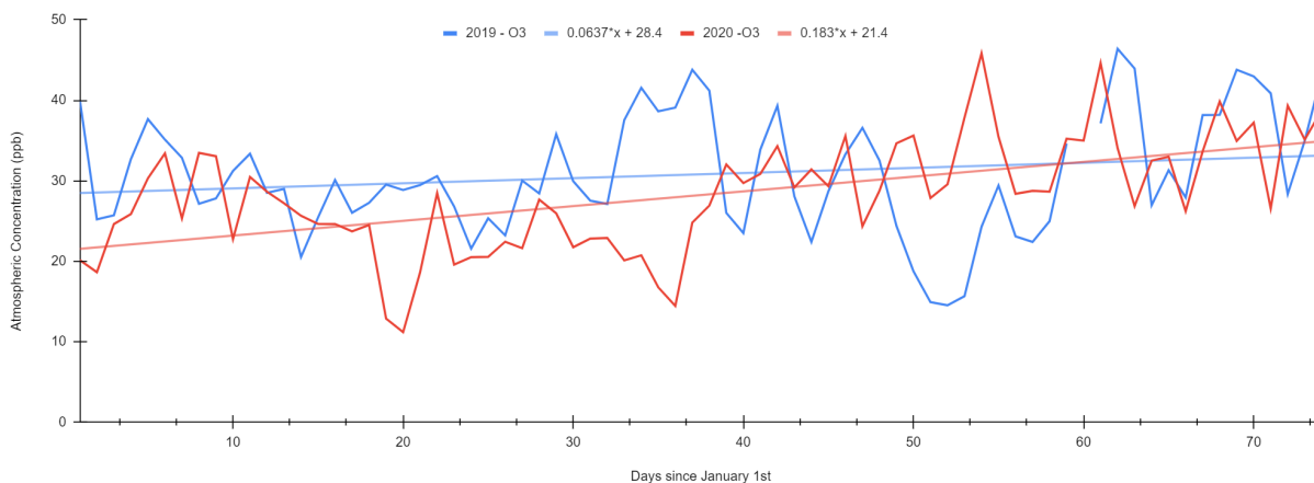
Figure 3. Graph of the averages of atmospheric concentrations in the city. Date shown in days since January 1. Own elaboration with data from the RAMA.
