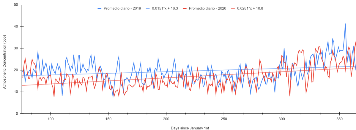
Daily averages of Nitrogen Dioxide in Mexico City from March 15 to December 31, 2020 and 2019
