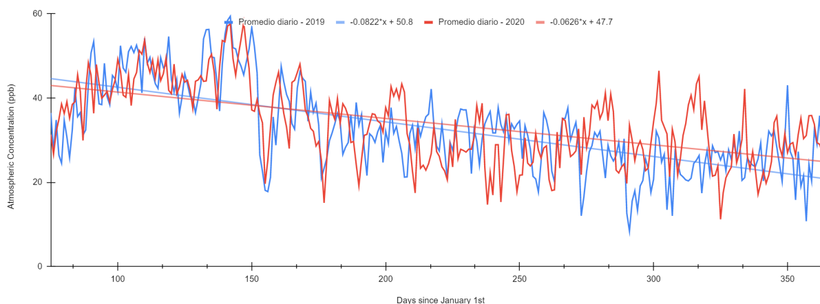
Figure 4. Graph of the averages of atmospheric concentrations in the city. Date shown in days since January 1. Own elaboration with data from the RAMA.
