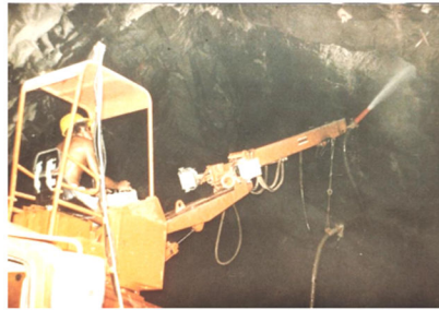
Figure 9 Shotcrete spraying process using 'roboshot' (Hoek, 1993)
