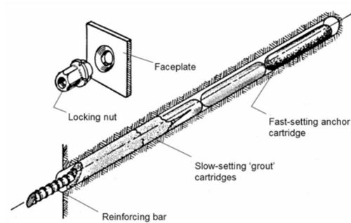
Figure 4 Illustration of resin grout bolt application (Hoek, 1993)
