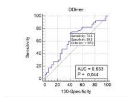
Figure 1. ROC curve of D-Dimer levels as mortality predictor.
