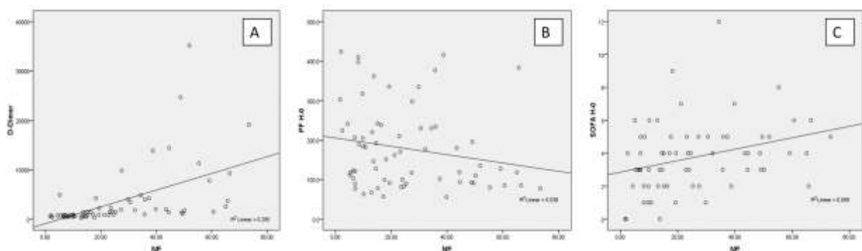
Fig.1. Scatterplot diagram of the correlation of NE serum levels towards (A) D-Dimer, (B) \text{PaO}_2/\text{FiO}_2 ratio, and (C) SOFA score
