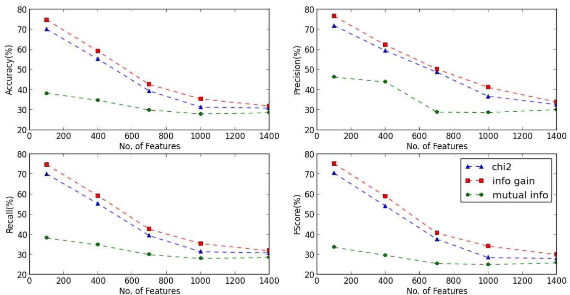
KNeighborsClassifier
