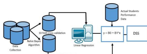
Figure 1. General Architecture for Classification using Naïve Bayes Algorithm for Students Performance
