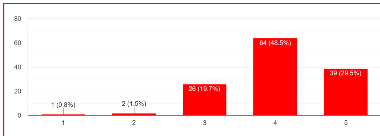
Fig. 10. Understandability
