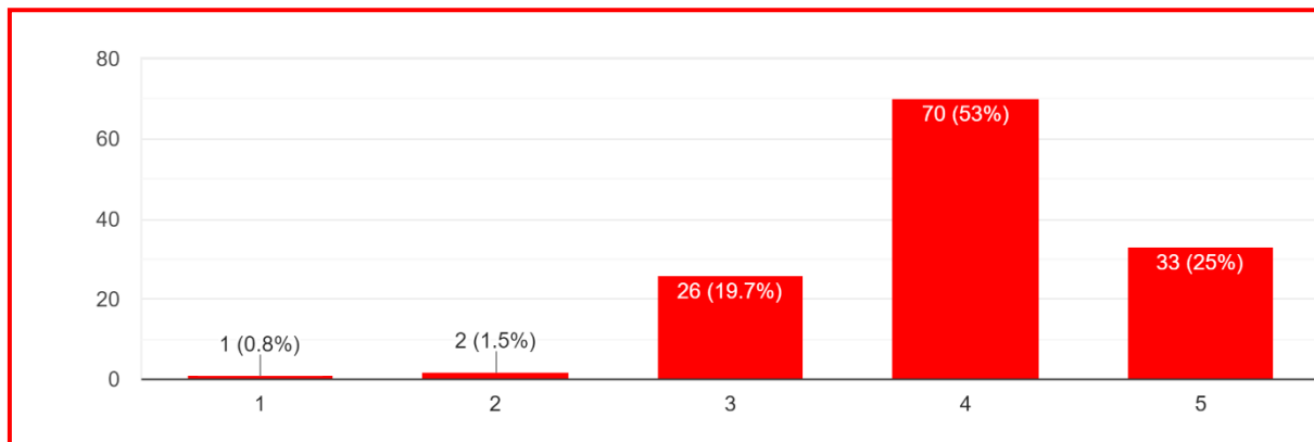
Fig. 6. Accurateness
