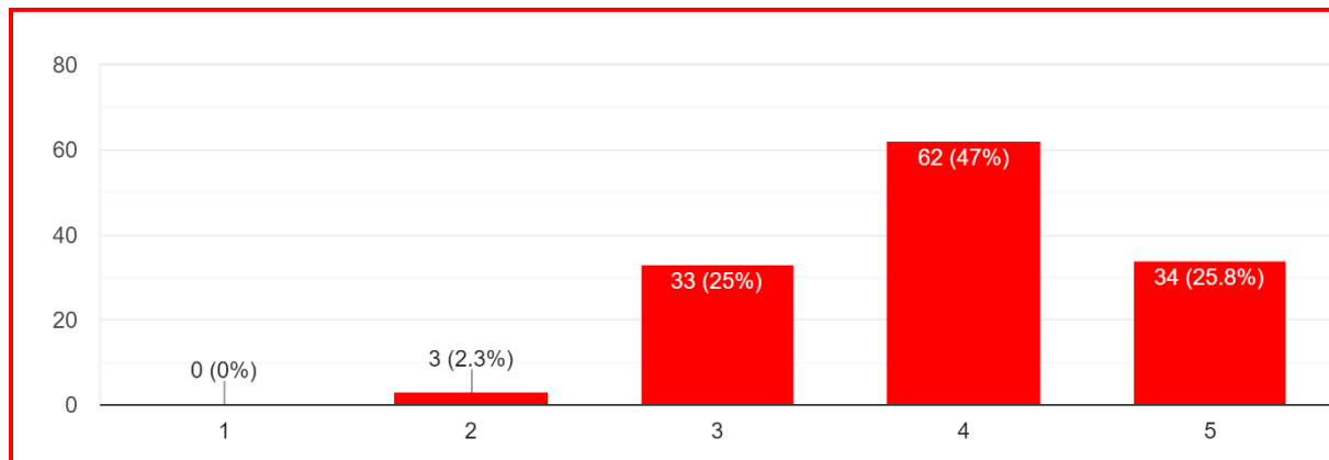
Fig. 9. Recoverability
