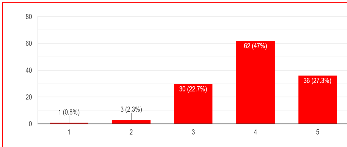
Fig. 12. Testability
