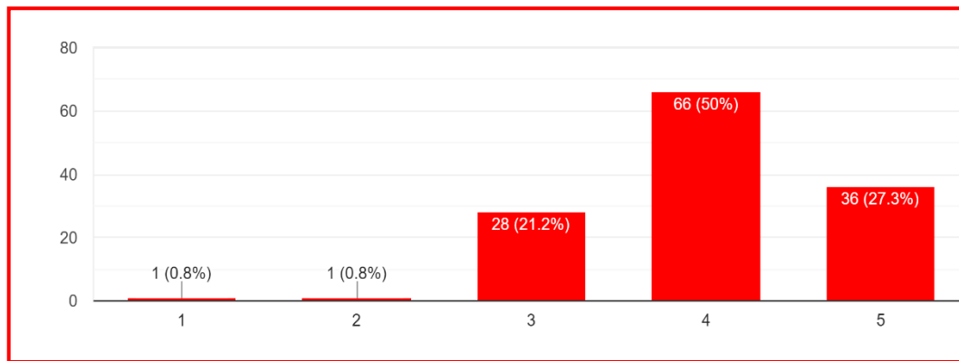
Fig. 11. Changeability
