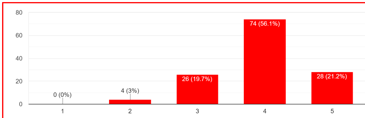
Fig. 7. Interoperability
