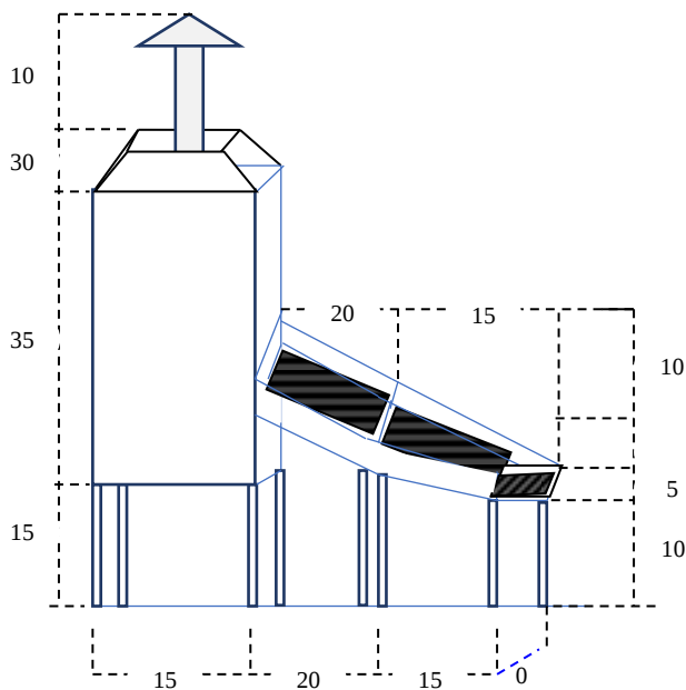
Fig 2. Dimensions of natural convection solar dryer (Not to scale)
