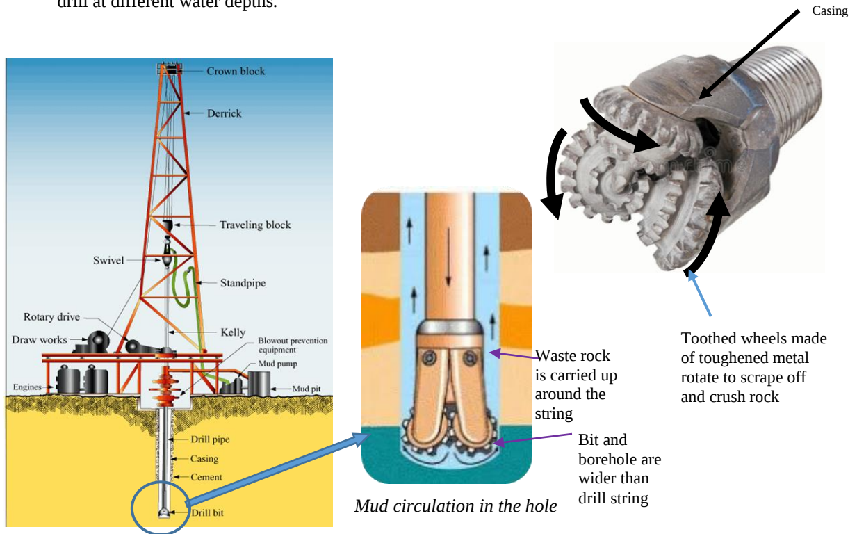
Fig. 4: Petroleum onshore drilling rig – picture from internet adapted with additional illustrations
