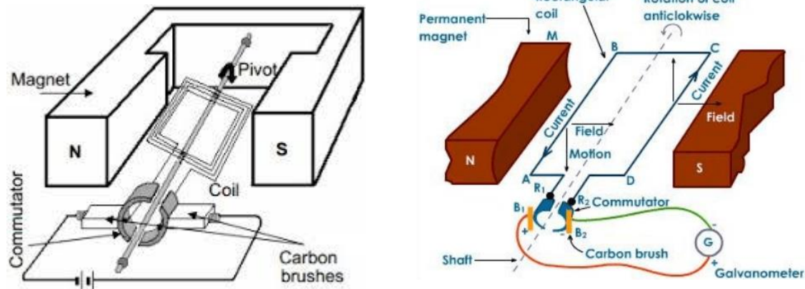
Fig. 13: Working principle of an electric generator
