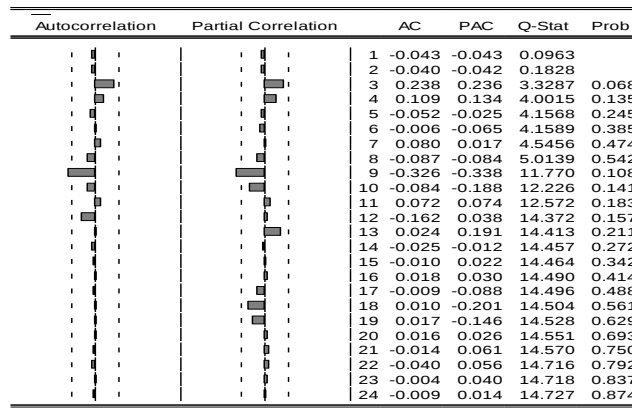
Fig. iv: Correlogram of Residuals
