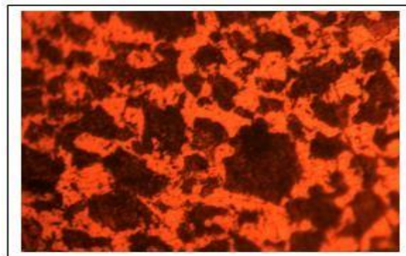
Fig. 11 Photomicrograph of sample C, annealed at 850^{\circ}\text{C}
