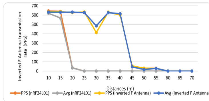
Graph 2. Inverted F Antenna transmission rate (Packet per second) vs. Distance.
