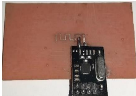
Figure 7. The AN043 PCB antenna
