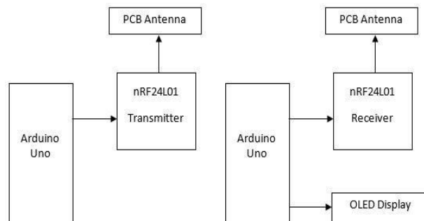
Figure 3. Block diagram
