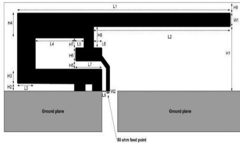
Figure 8. IFA Dimensions.
