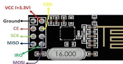
Figure 1. nRF24L01 [3].
