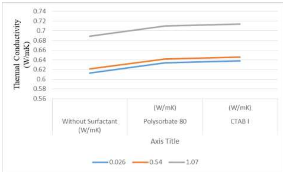
Figure 5 Thermal Conductivity of Nanofluids
