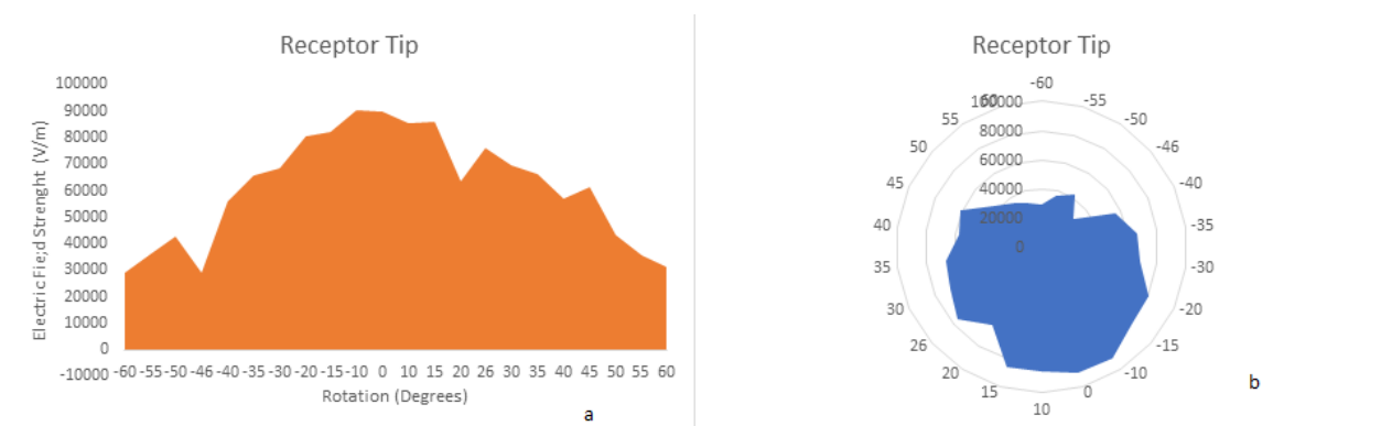
Figure 7. The (a) Area and (b) Radar plots for the electric field distribution on the receptor tip
