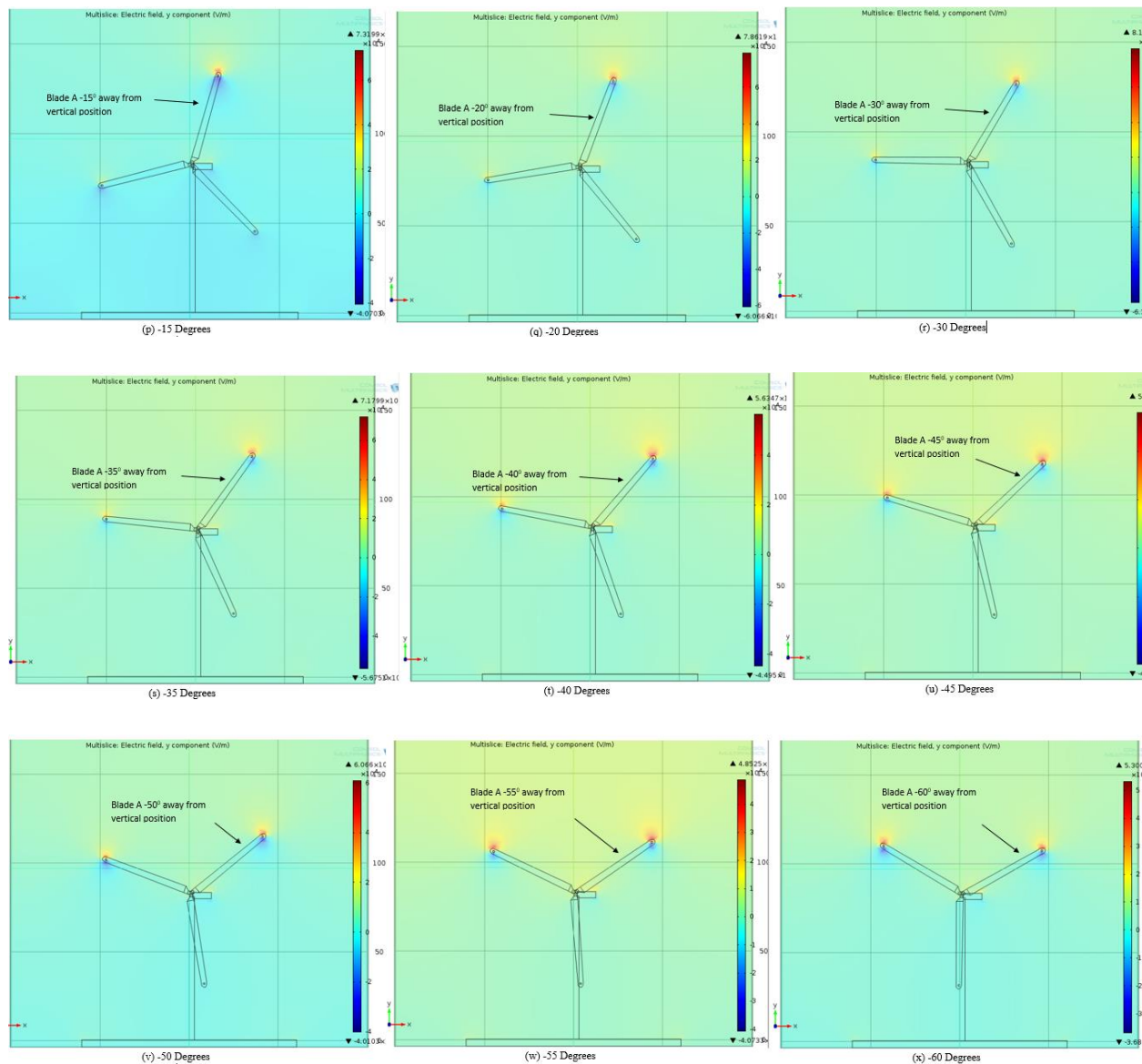
Figure 3. maximum electric field distribution due to cloud charge as blade A is rotated from -60 to +60 degrees from the vertical position.
