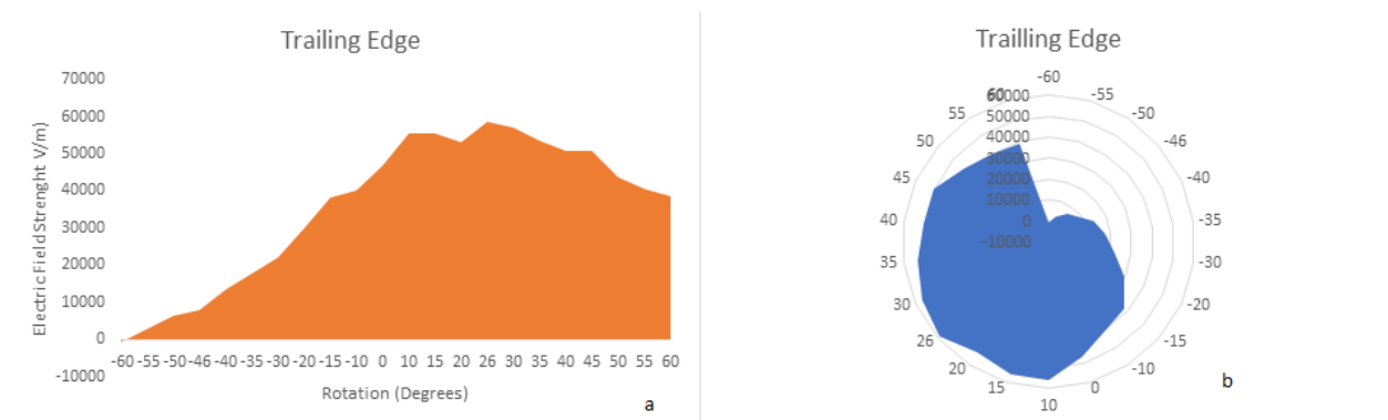
Figure 6. The (a) Area and (b) Radar plots for the electric field distribution on the surface of the blade trailing edge
