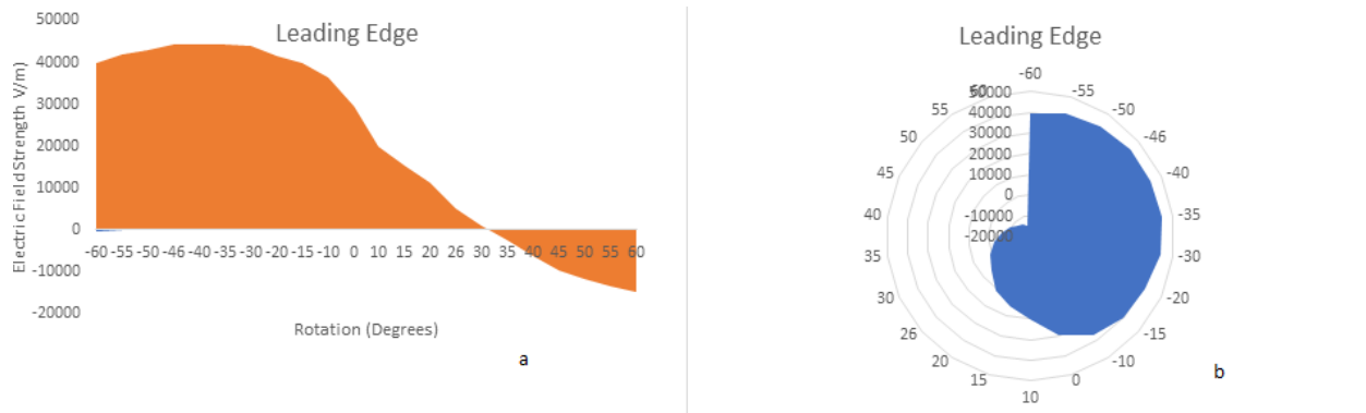
Figure 5. The (a) Area and (b) Radar plots for the electric field distribution on the surface of the blade leading edge
