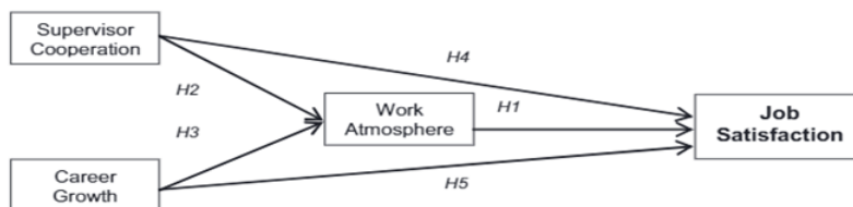
Figure 1: Conceptual Framework
