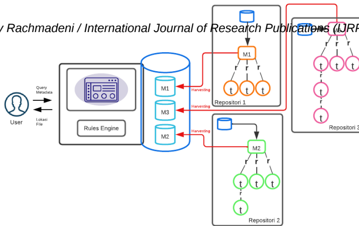
Figure. 3. the association between ontology and rules engine.
