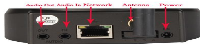
Figure 5: Back view of an IP Camera
