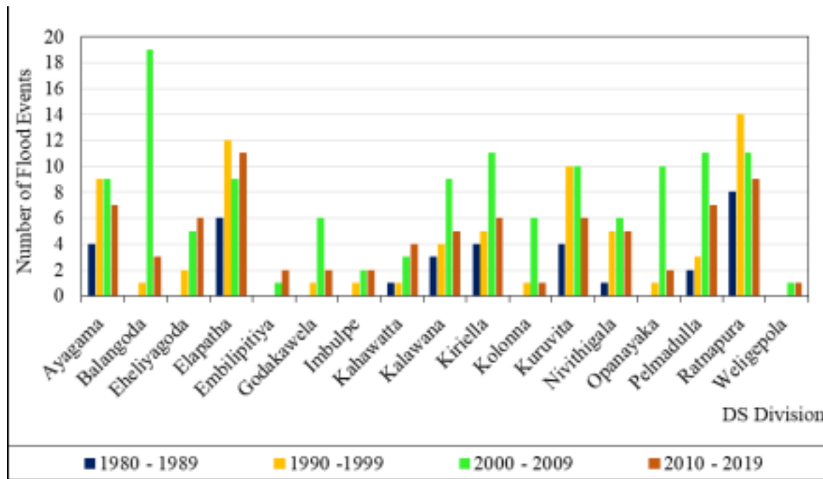
Fig. 9. Decadal Wise Flood Frequency of Divisional Secretariat (DS) Divisions in the Rathnapura District (Source: EM-DAT database, 2021)
