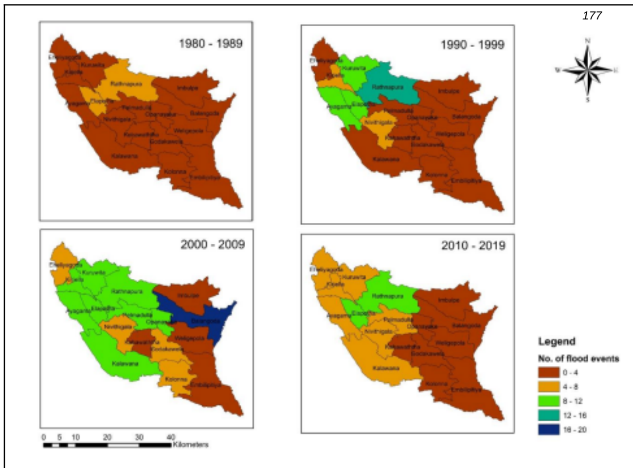
Fig. 10. Spatial Distribution of Flood Events in Rathnapura District
