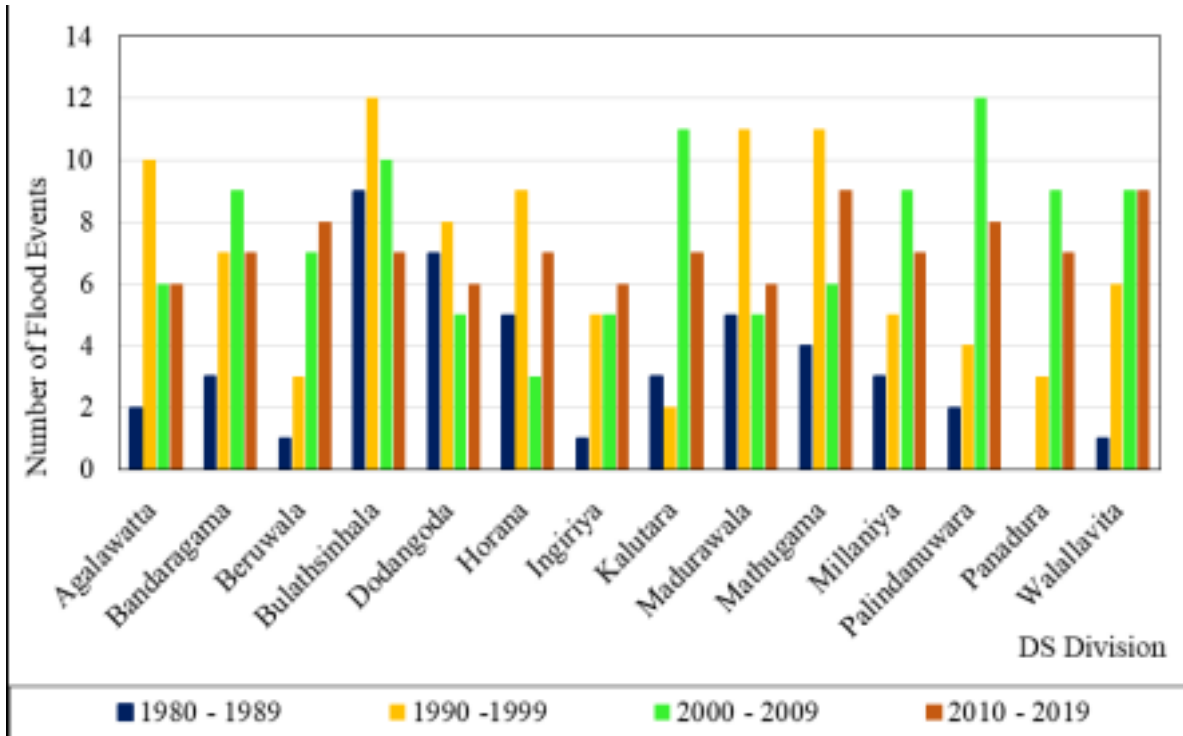
Fig. 5. Decadal Wise Flood Frequencies of Divisional Secretariat Divisions in the Kalutara District (Source: EM-DAT database, 2021)
