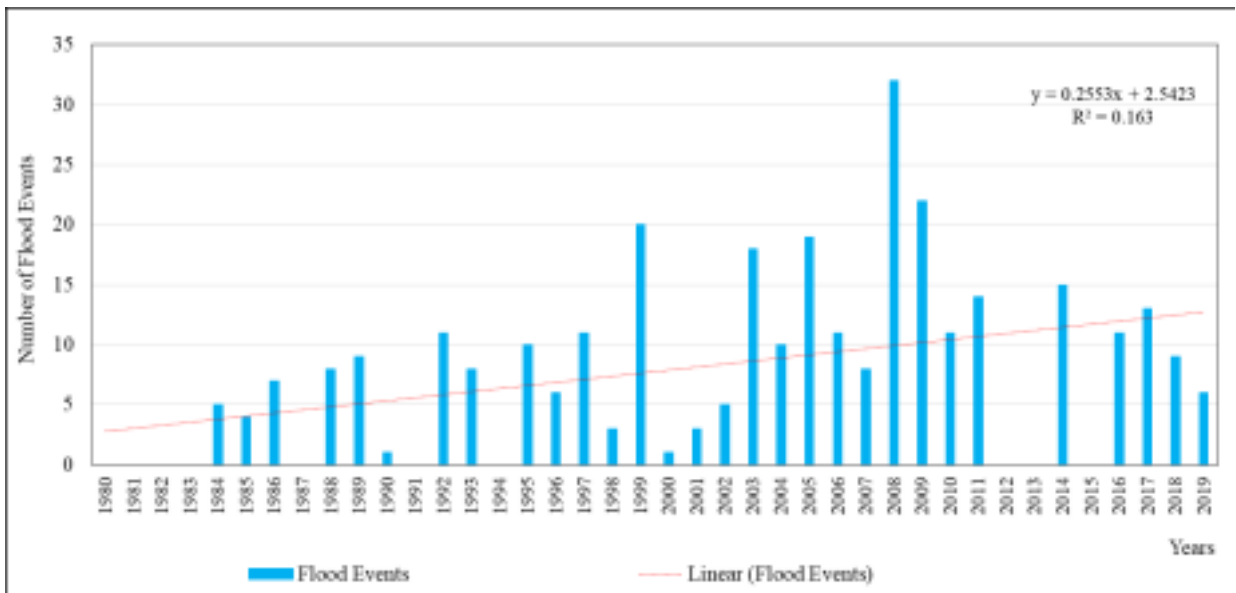
Fig. 8. Trend of Flood Events in Rathnapura District (Source: EM-DAT database, 2021)
