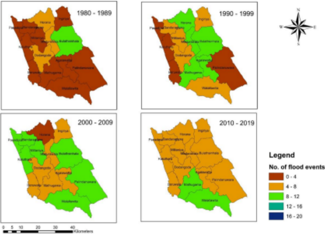
Fig. 6. Spatial Distribution of Flood Events in Kalutara District
