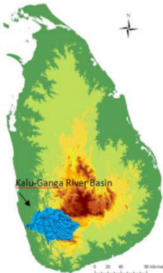
Fig. 2. Kalu-Ganga River Basin (Source: Samarasinghe, et al. (2021))
