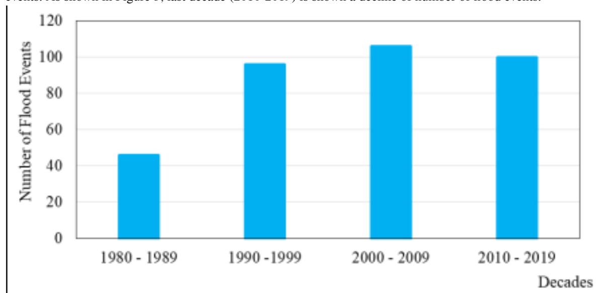
Fig. 3. Total Number of Flood Events in Kalutara District (Source: EM-DAT database, 2021)
