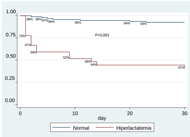
Figure 2 Kaplan Meier Survival Estimation Curve 30-day Post-IMA Mortality Curve Based on Hyperlactatemia
