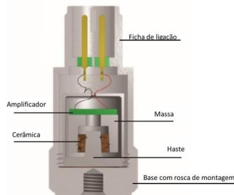
Picture 3(c) accelerometer (DMC)
