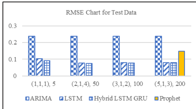
Fig. 6: RMSE Chart for Test Data
