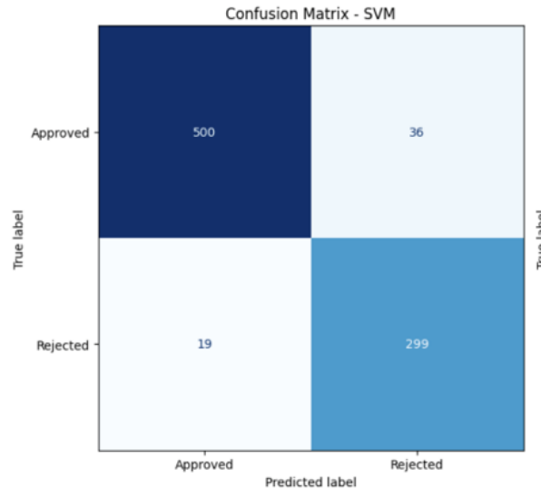
Figure 3: Confusion Matrix for Best Model
