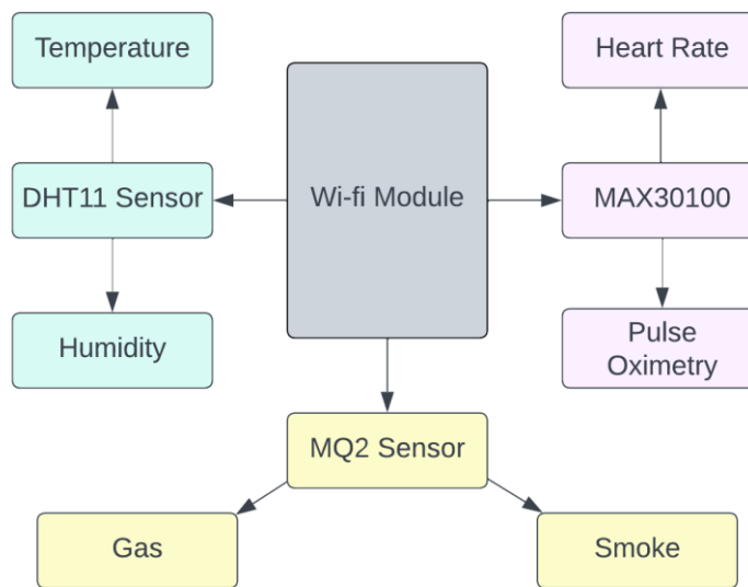
Fig. 1. Block Diagram
