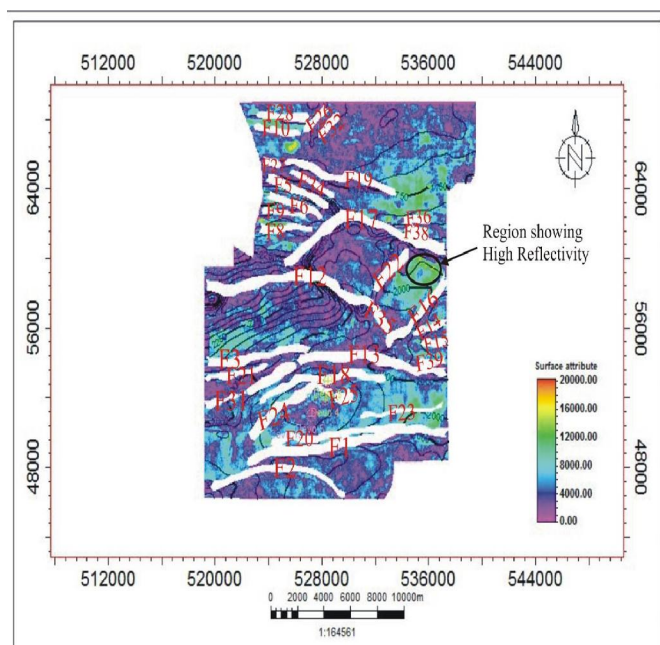
Fig. 3.11c: RMS Surface Attribute Showing on Horizon 3
