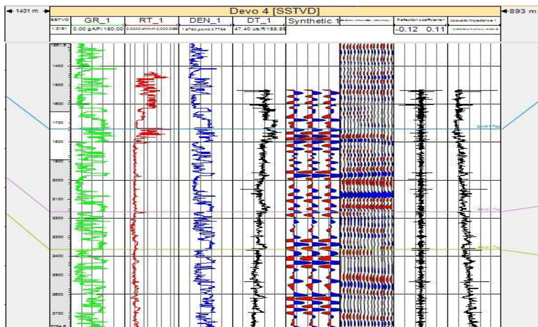
Fig. 3.3: Well-to-Seismic Tie on DEVO-4 Well
