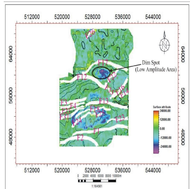
Fig. 3.10b: Mean Amplitude Surface Attribute Showing on Horizon 2
