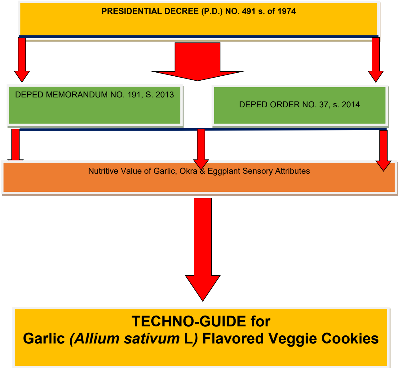
Figure 1. Conceptual Framework
