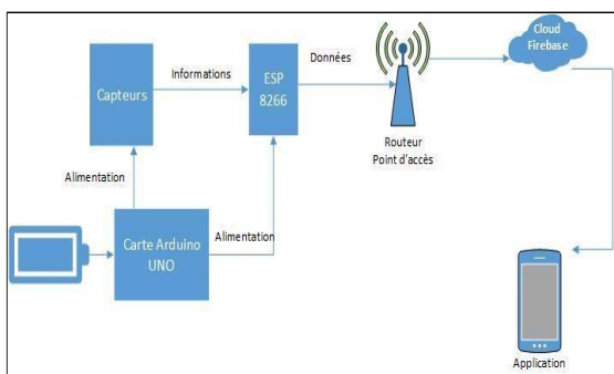
Figure 6: functional scheme
