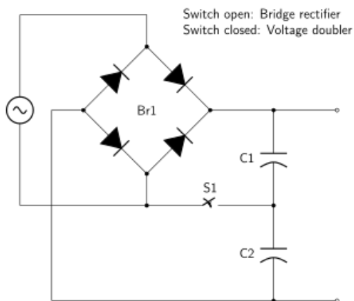
Figure 5: Rectifier
