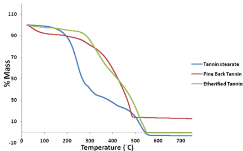
Figure 7. TGA thermograms of pine bark tannin (PBT), PBT stearate and etherified tannin. Increasing the onset temperature of degradation is beneficial for high temperature processing or applications. For instance, the incorporation of modified tannins into thermoplastics, which often requires temperatures above 180 °C to process with thermoplastics, namely, polyethylene or polypropylene.
